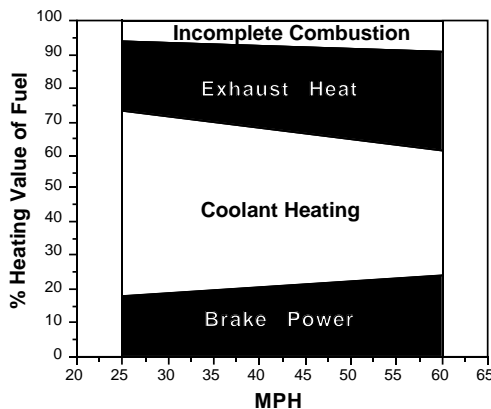
Combustion Heat Distribution
